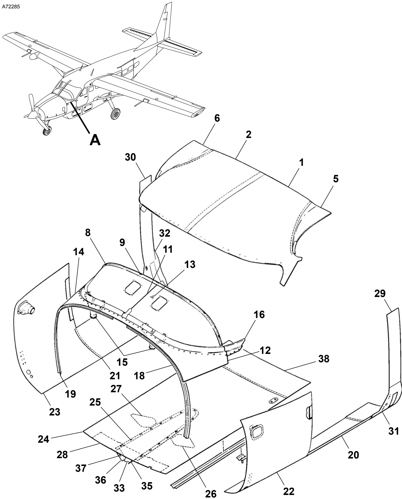
FORWARD FUSELAGE SKINS AND COMPONENTS Figure 04. (Sheet 1)
