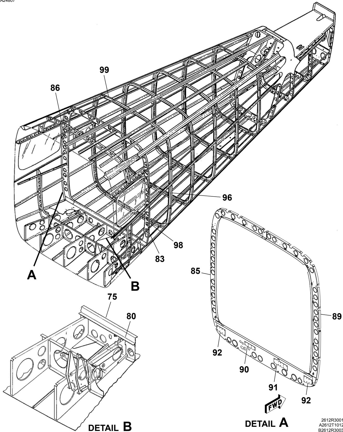
TAILCONE STRUCTURE Figure 01. (Sheet 2)
