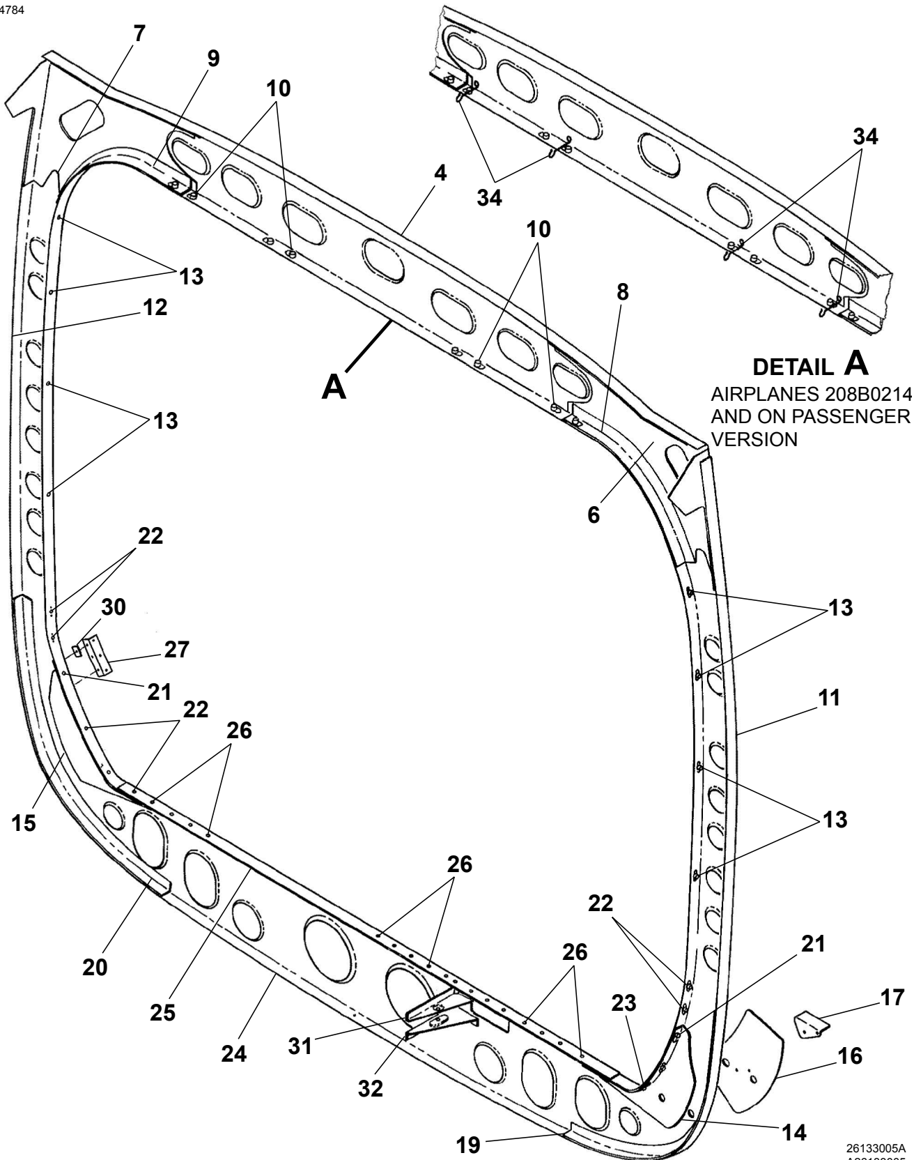
BULKHEAD ASSEMBLY - FS 166.45 Figure 01. (Sheet 1)
