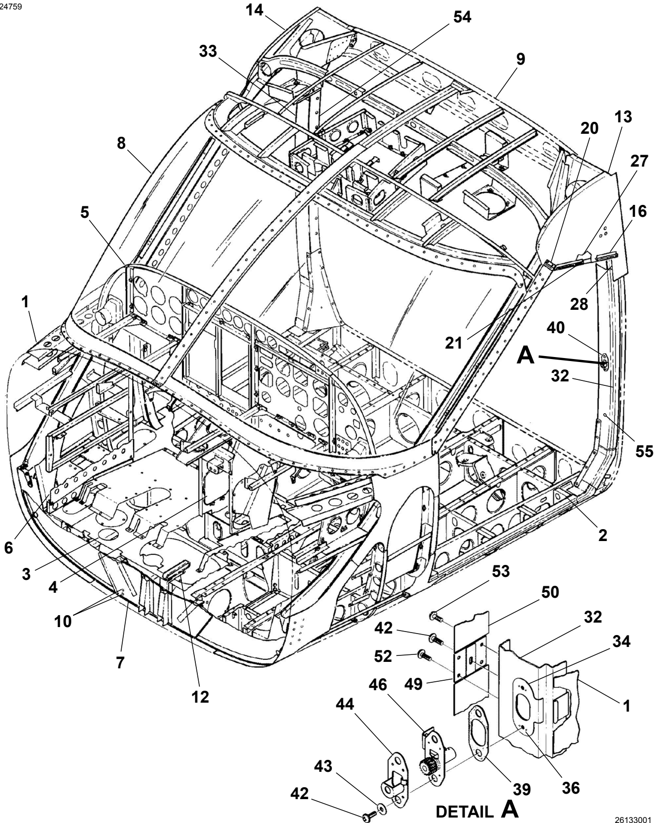
FORWARD FUSELAGE STRUCTURE Figure 02. (Sheet 1)
