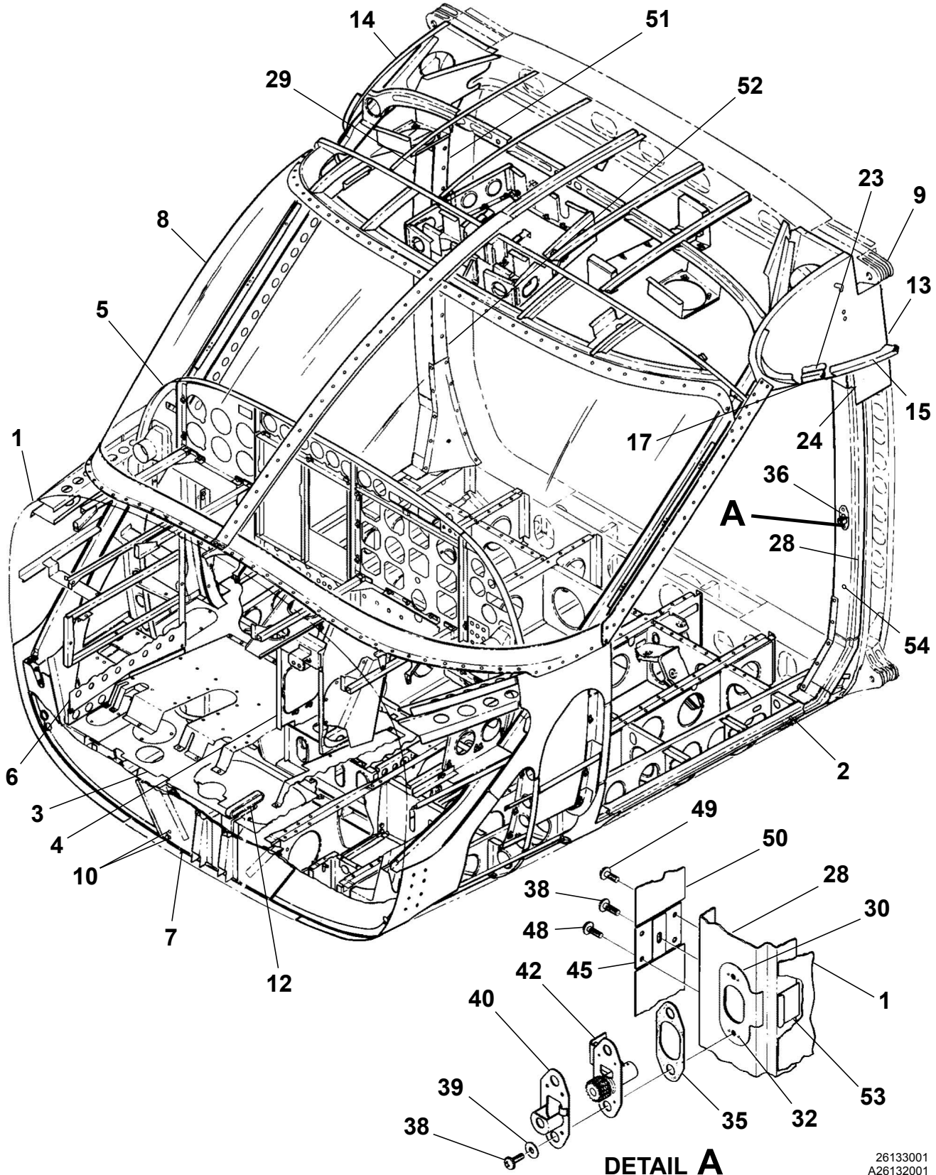
FORWARD FUSELAGE STRUCTURE Figure 01. (Sheet 1)
