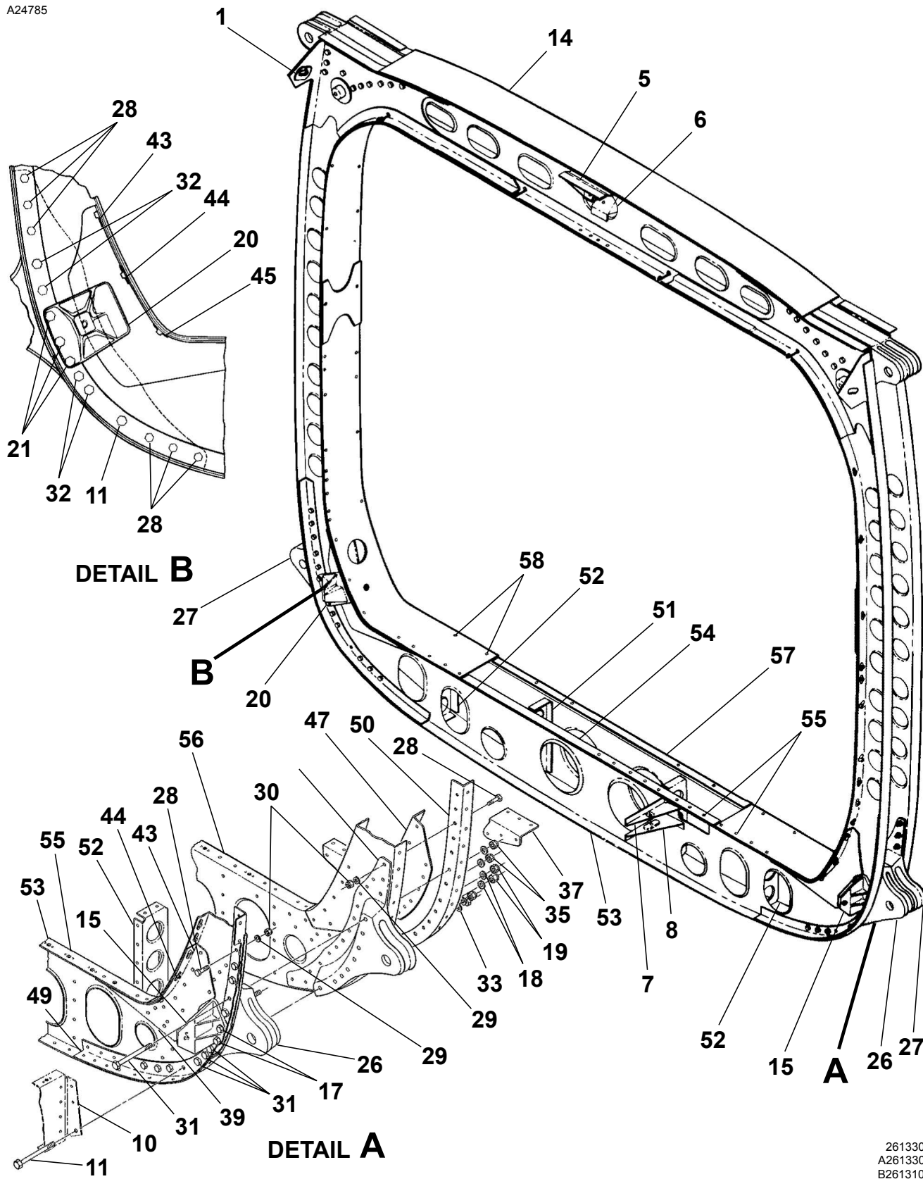
FORWARD CARRY THRU STRUCTURE Figure 02. (Sheet 1)
