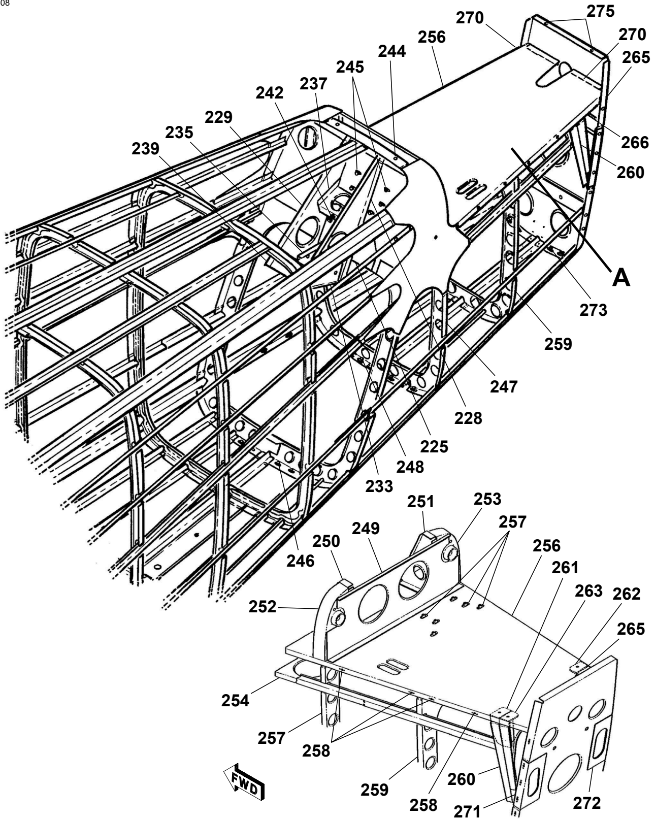
DETAIL A TAILCONE STRUCTURE Figure 01. (Sheet 4)
