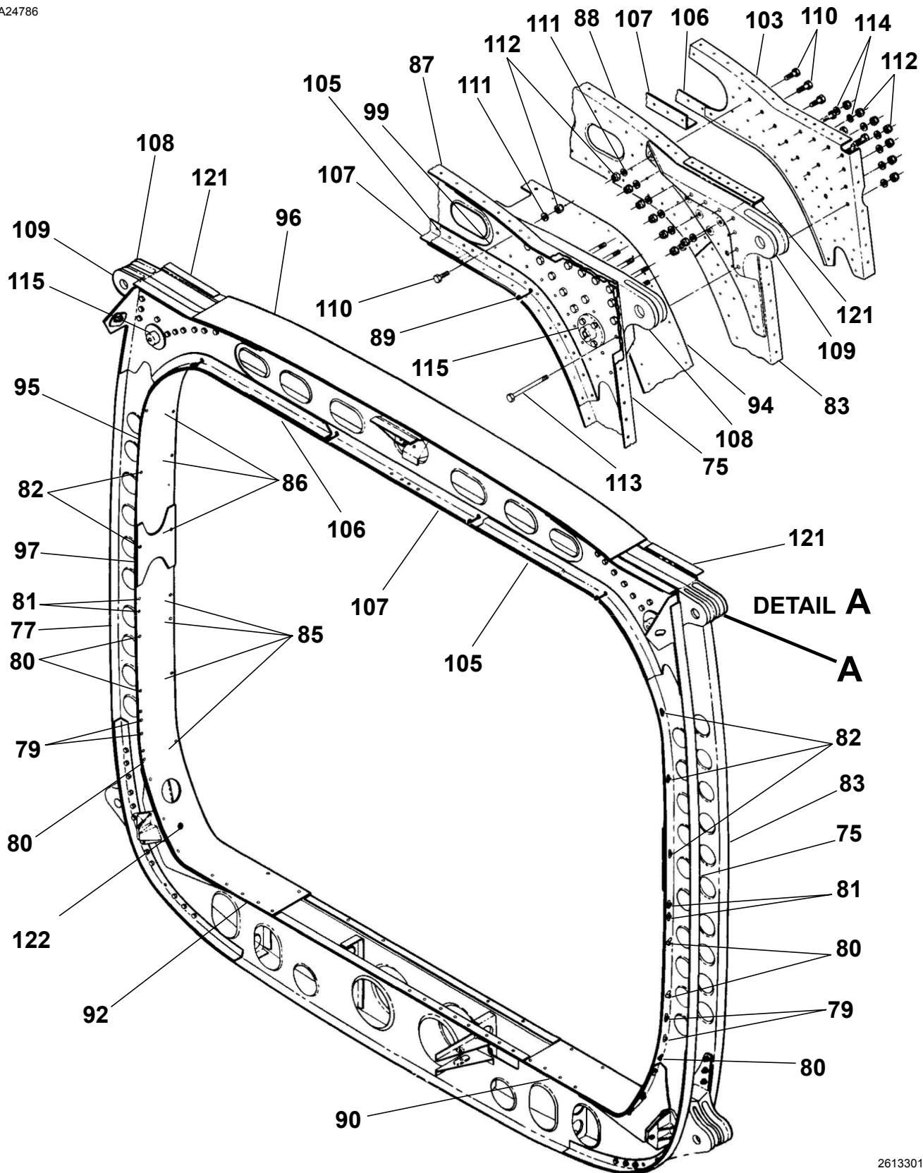
FORWARD CARRY THRU STRUCTURE Figure 02. (Sheet 2)
