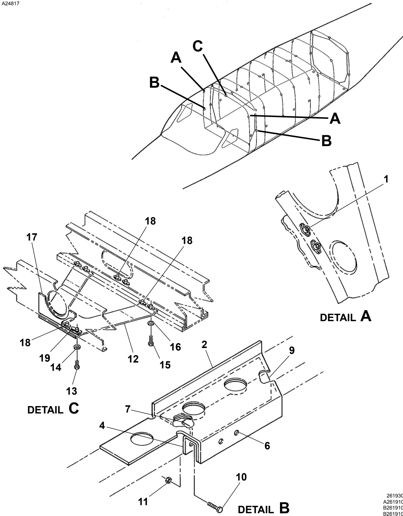
CARGO TIE DOWN STRUCTURE COMPONENTS Figure 02. (Sheet 1)
