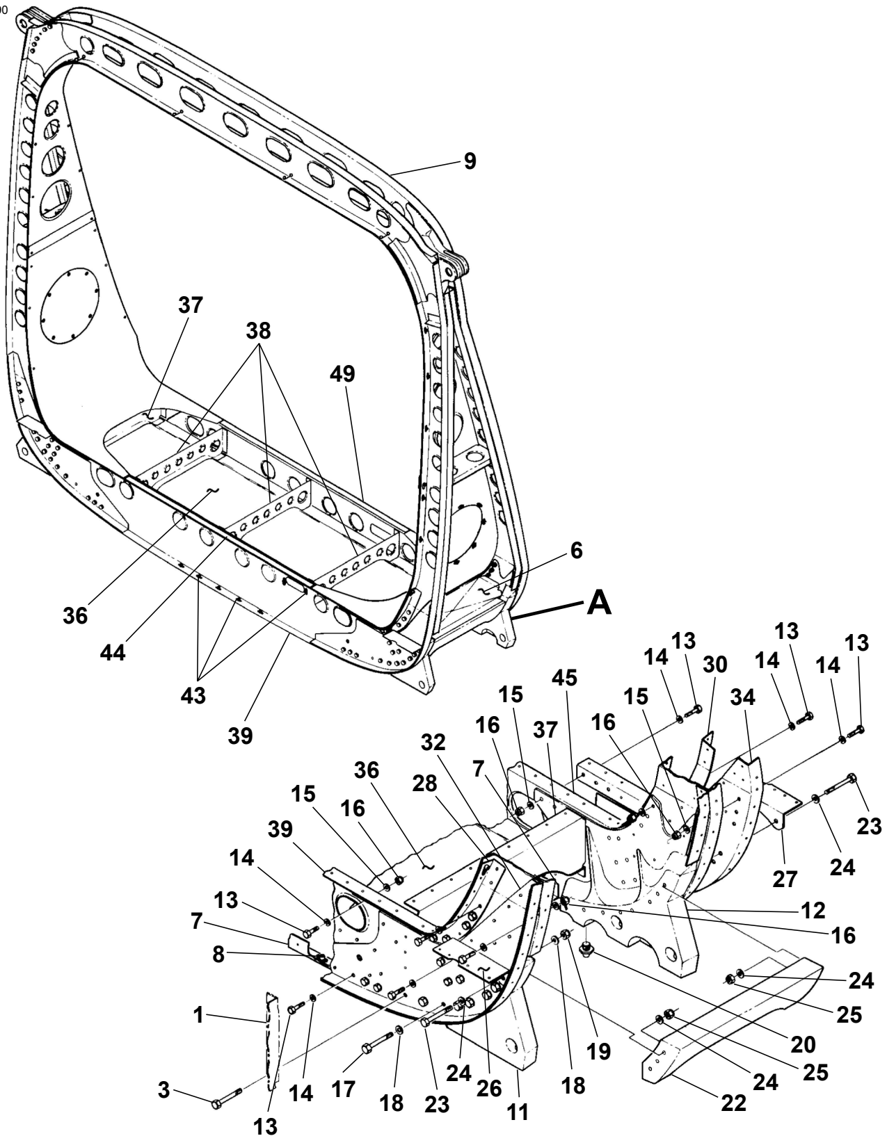
DETAIL A MAIN LANDING GEAR BULKHEAD STRUCTURE Figure 04. (Sheet 1)
