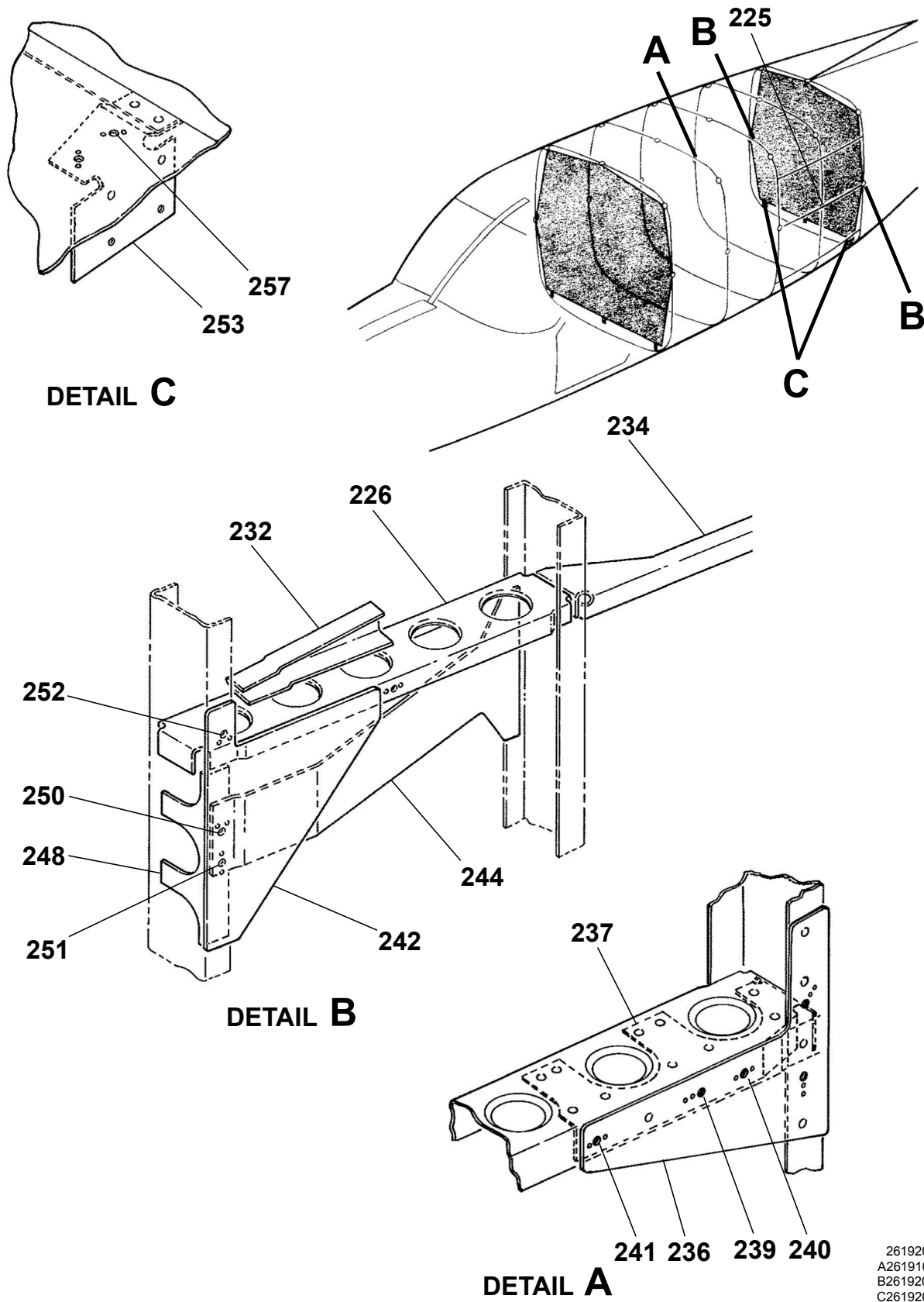
CARGO TIE DOWN STRUCTURE COMPONENTS CARGOMASTER Figure 01. (Sheet 4)
