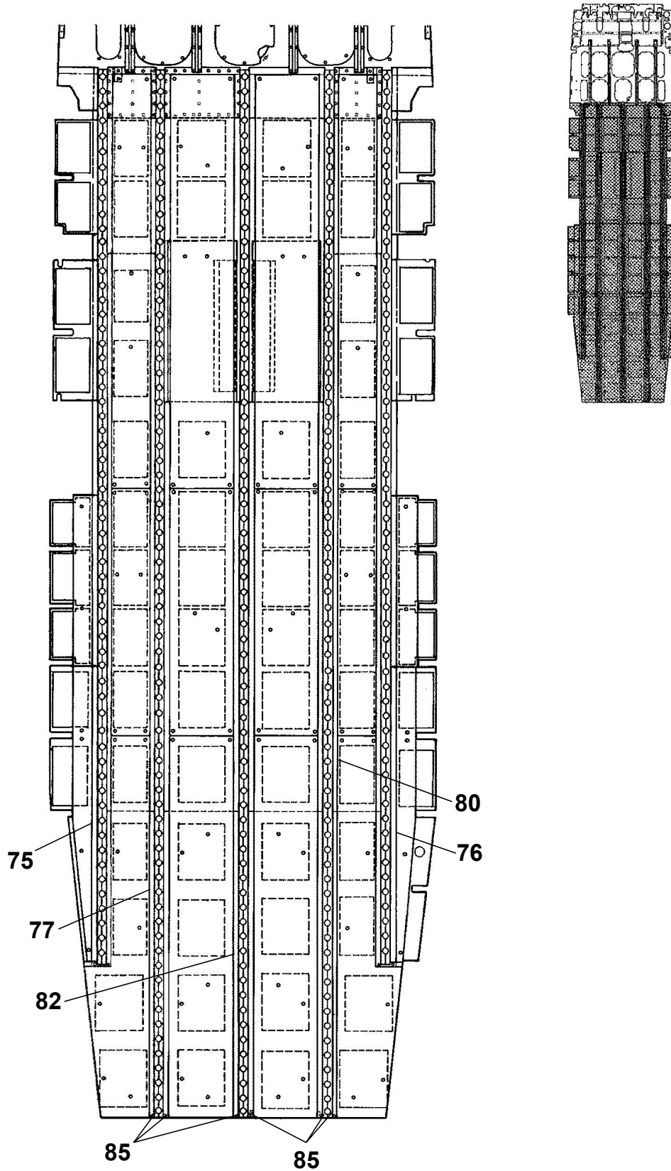
SEAT RAIL AND TRACK INSTALLATION Figure 02. (Sheet 2)
