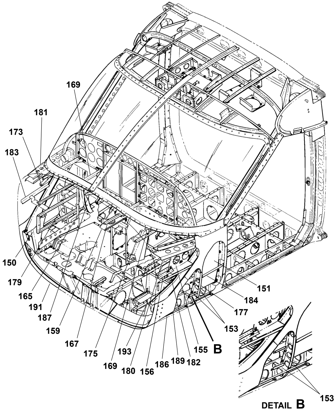
FORWARD FUSELAGE STRUCTURE Figure 01. (Sheet 3)
