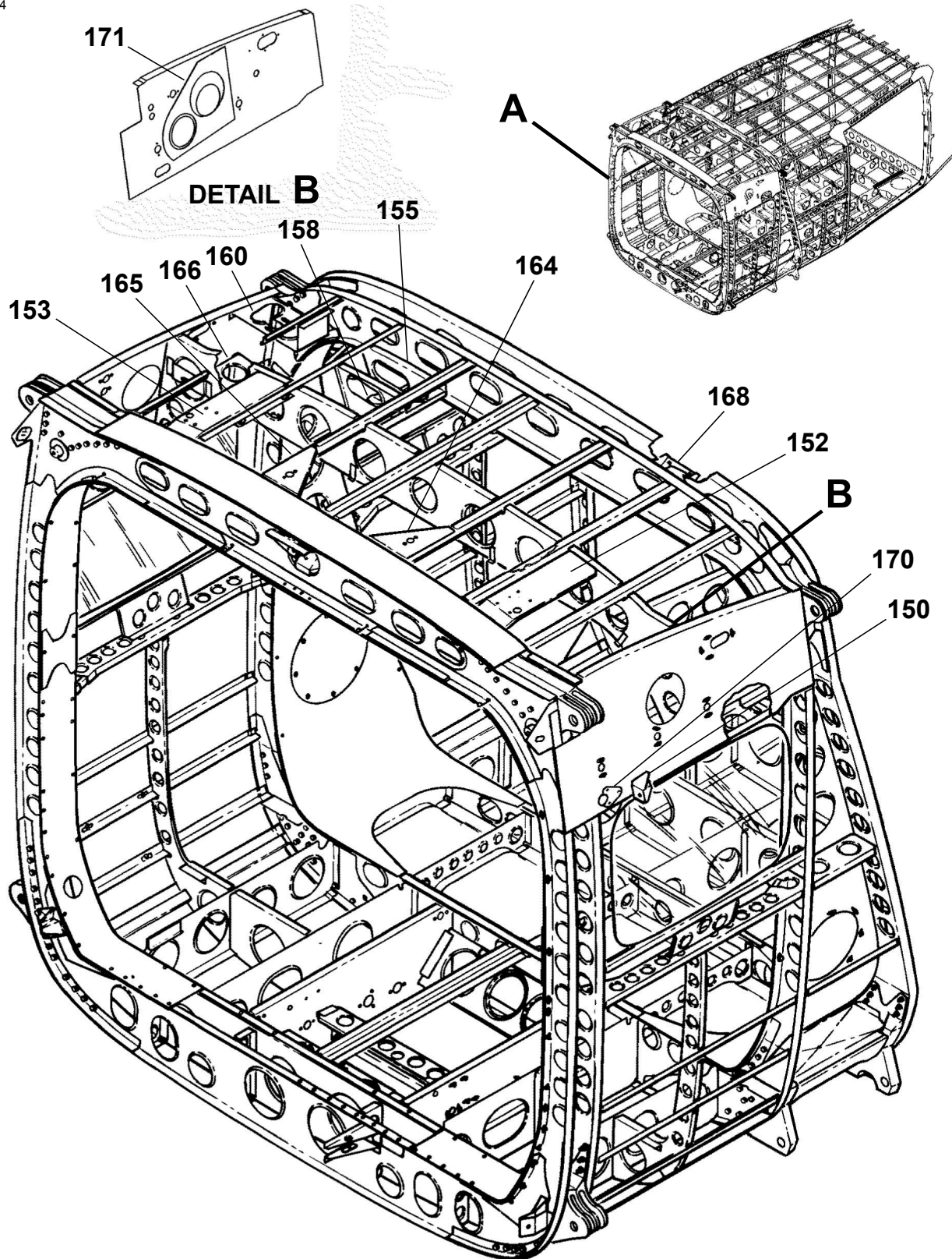
DETAIL A CENTER FUSELAGE STRUCTURE Figure 01. (Sheet 3)
