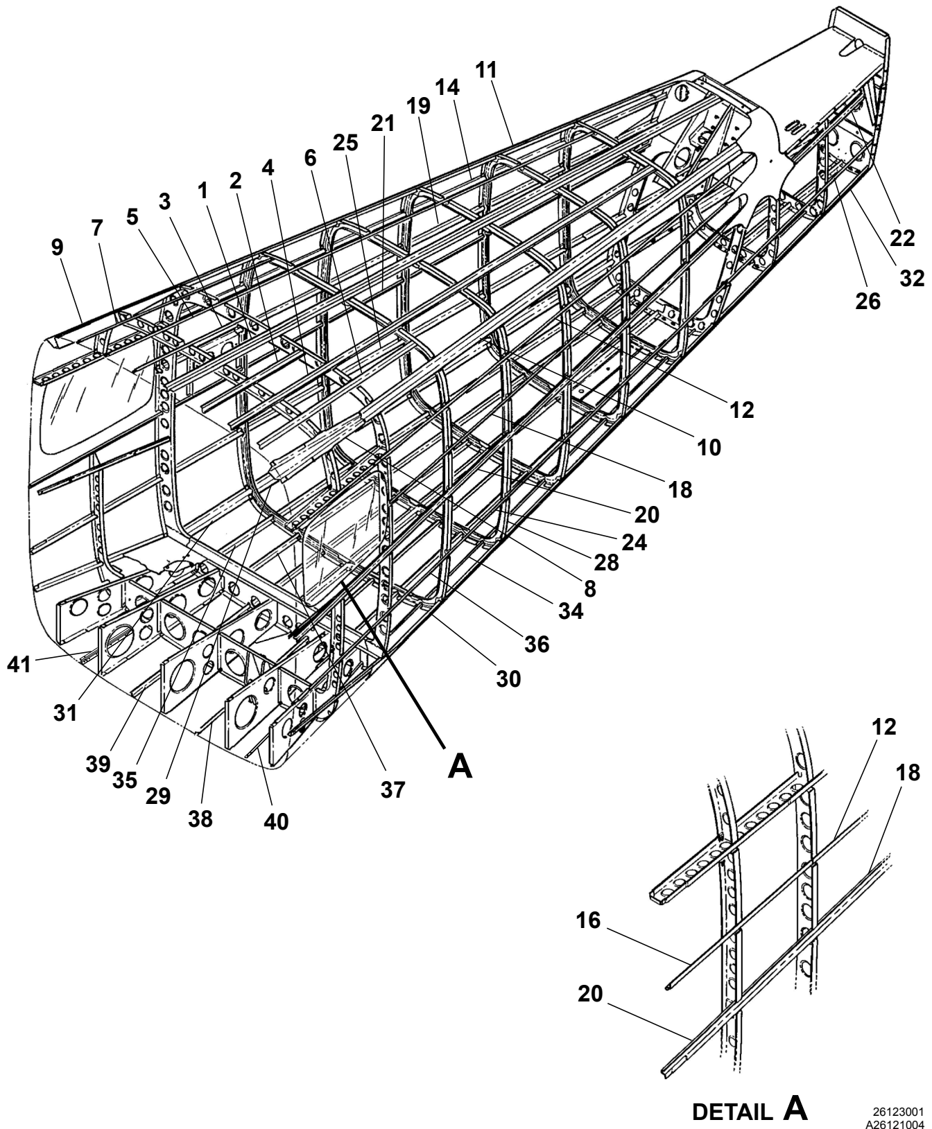
TAILCONE STRINGERS AND COMPONENTS Figure 03. (Sheet 1)
