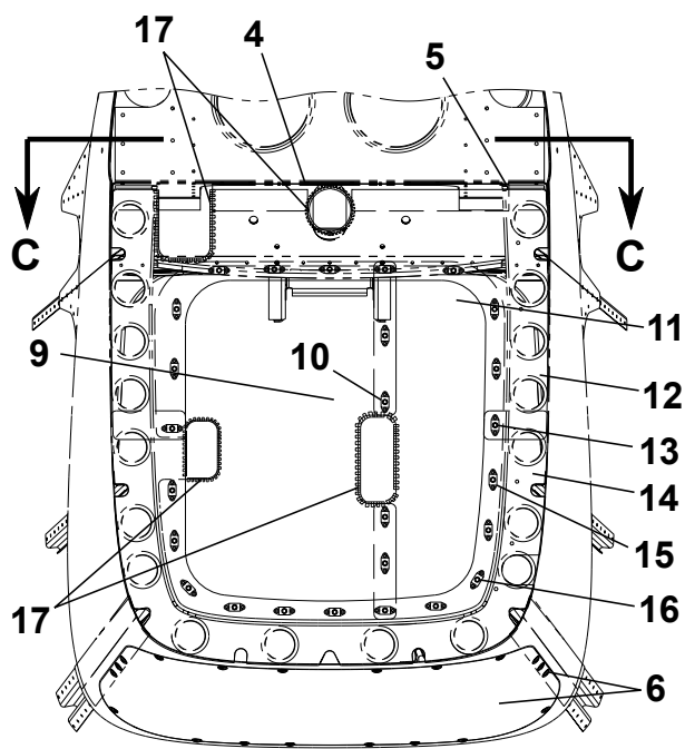
VIEW B-B
