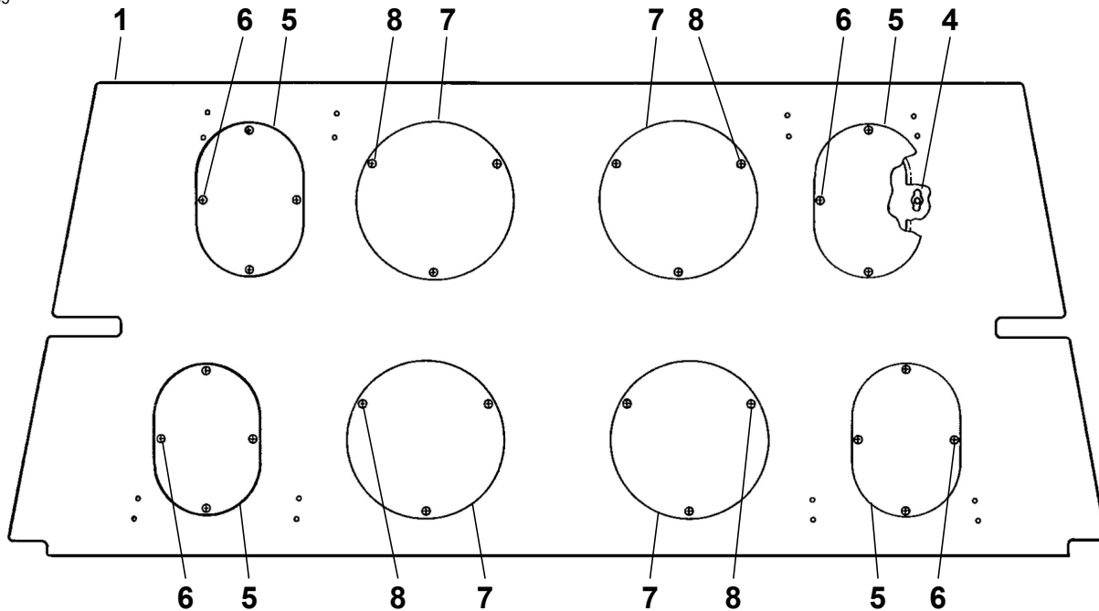
METAL FLOORBOARD
