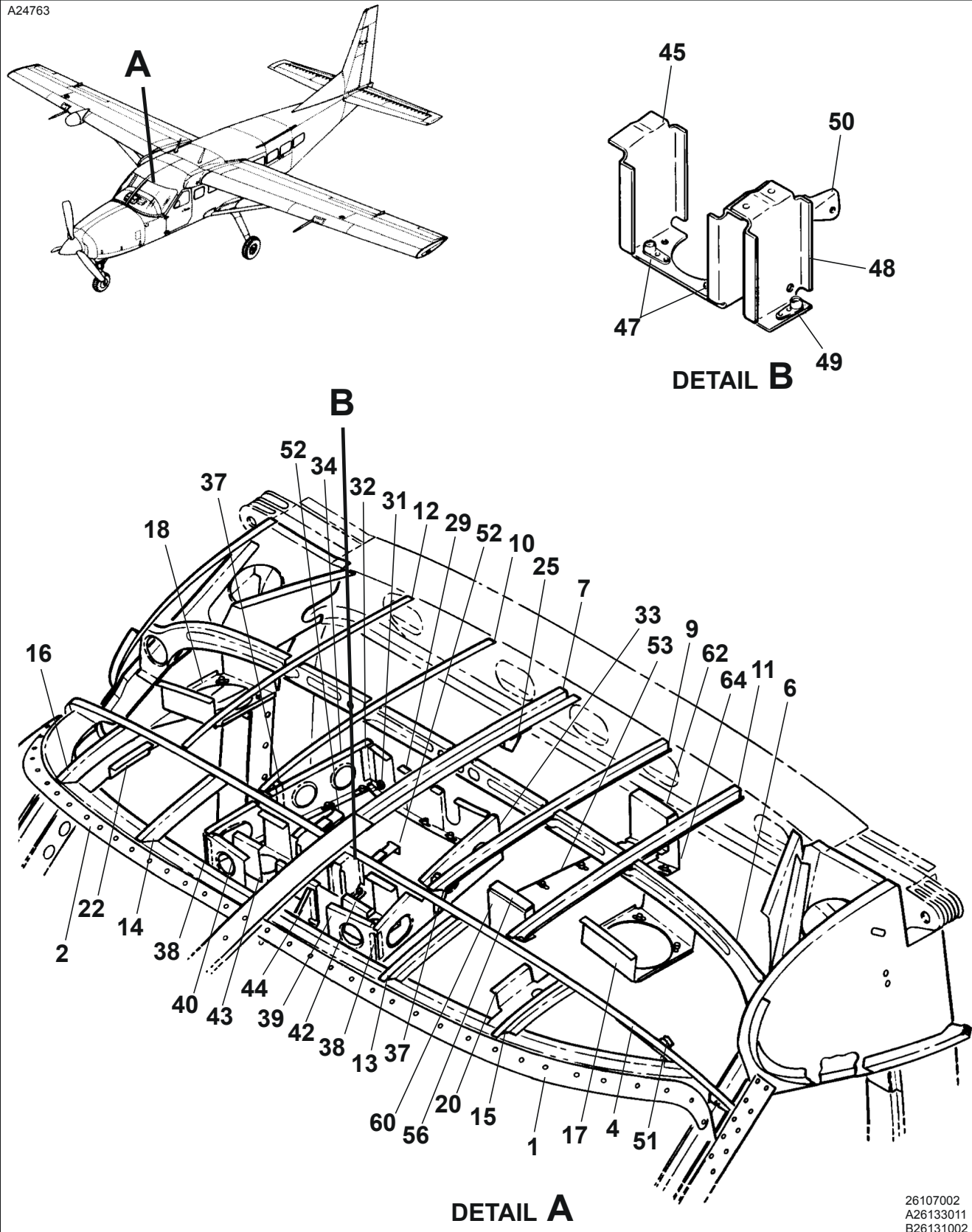
FORWARD CABIN TOP COMPONENTS Figure 01. (Sheet 1)
