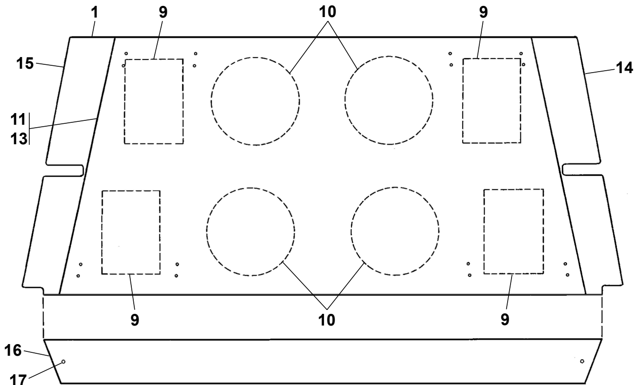
PLYWOOD FLOORBOARD
