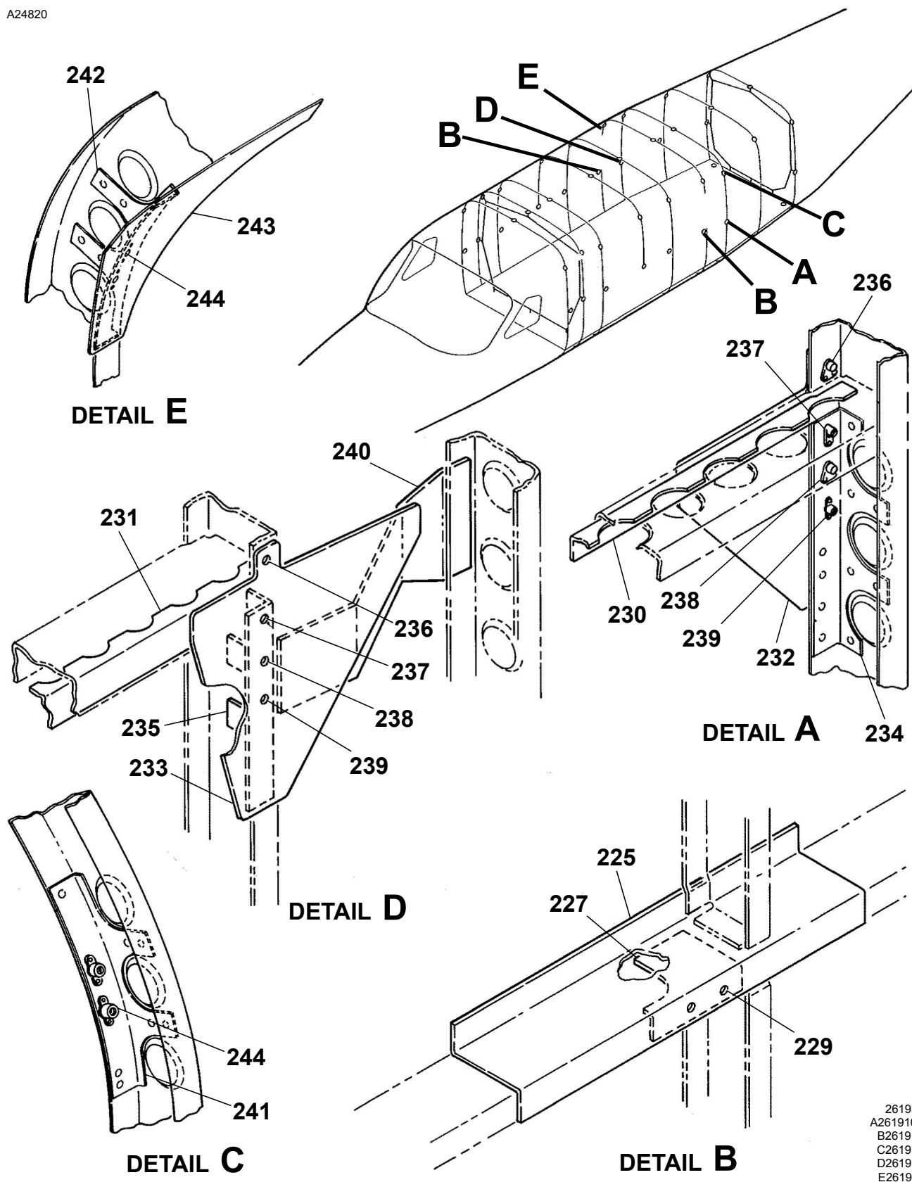
CARGO TIE DOWN STRUCTURE COMPONENTS Figure 02. (Sheet 4)
