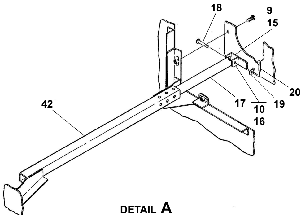
INSTRUMENT PANEL STRUCTURE Figure 05. (Sheet 1)
