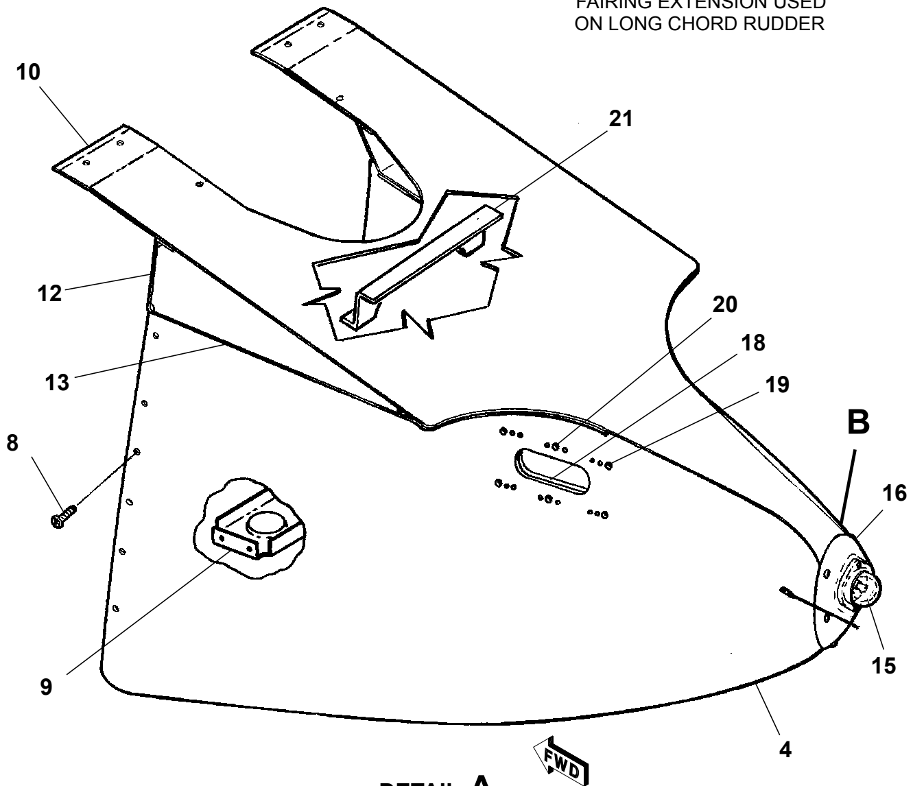
STINGER AND FAIRING ASSEMBLY Figure 01. (Sheet 1)
