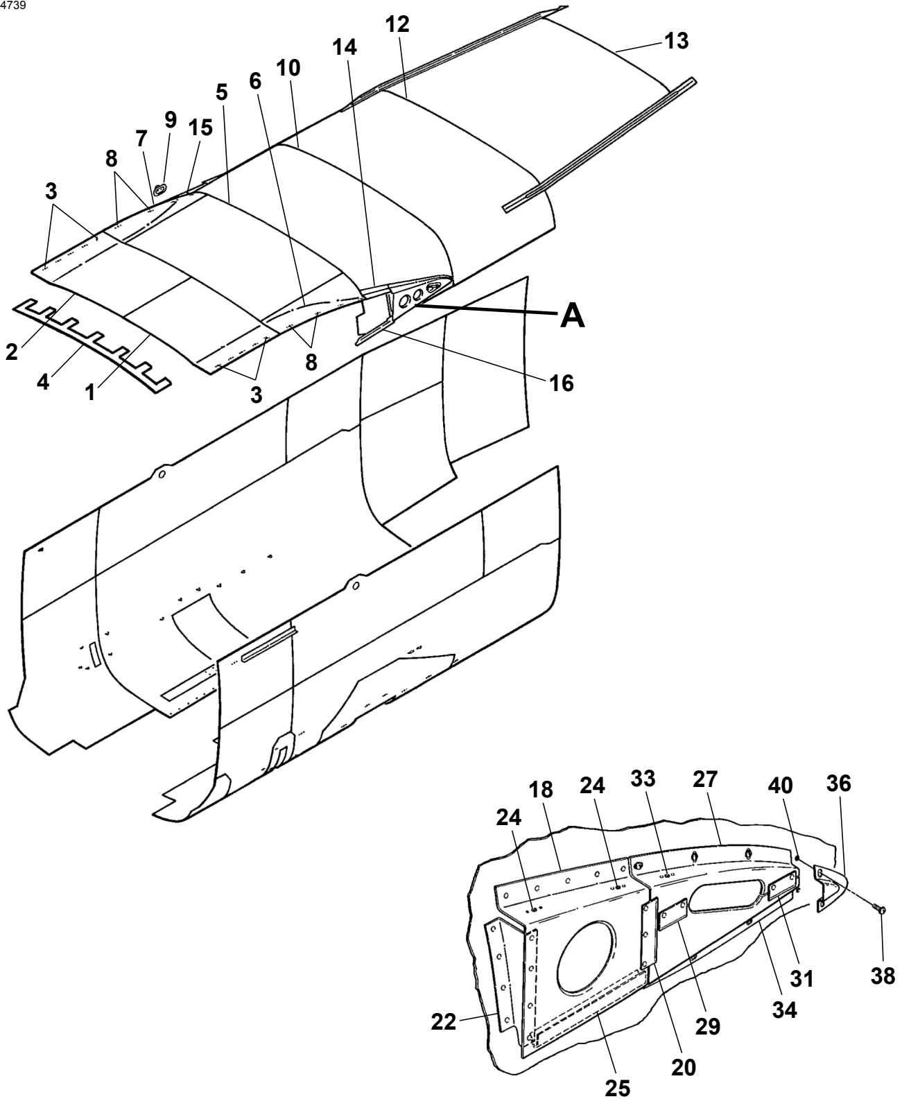
CENTER FUSELAGE SKINS AND COMPONENTS Figure 02. (Sheet 1)
