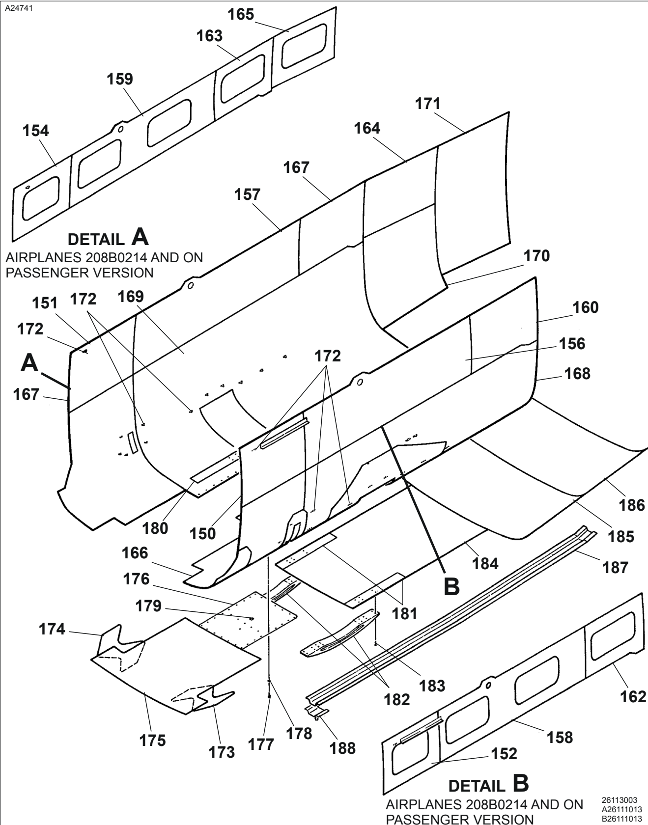
CENTER FUSELAGE SKINS AND COMPONENTS Figure 02. (Sheet 3)
