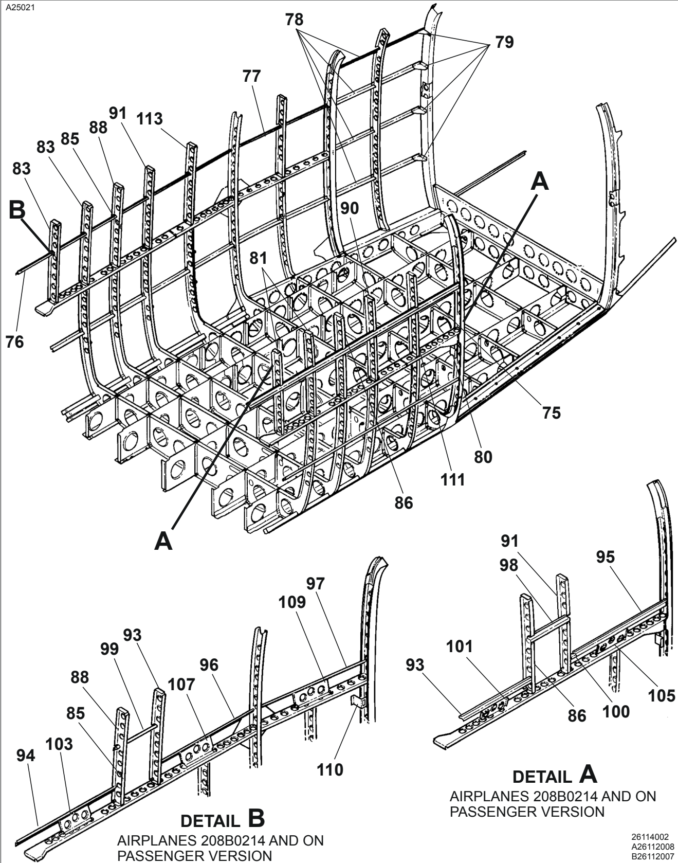
LOWER CENTER FUSELAGE STRUCTURE Figure 02. (Sheet 2)
