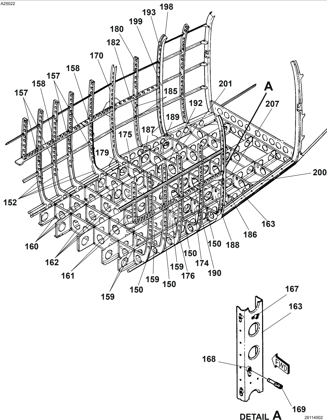
LOWER CENTER FUSELAGE STRUCTURE Figure 02. (Sheet 3)
