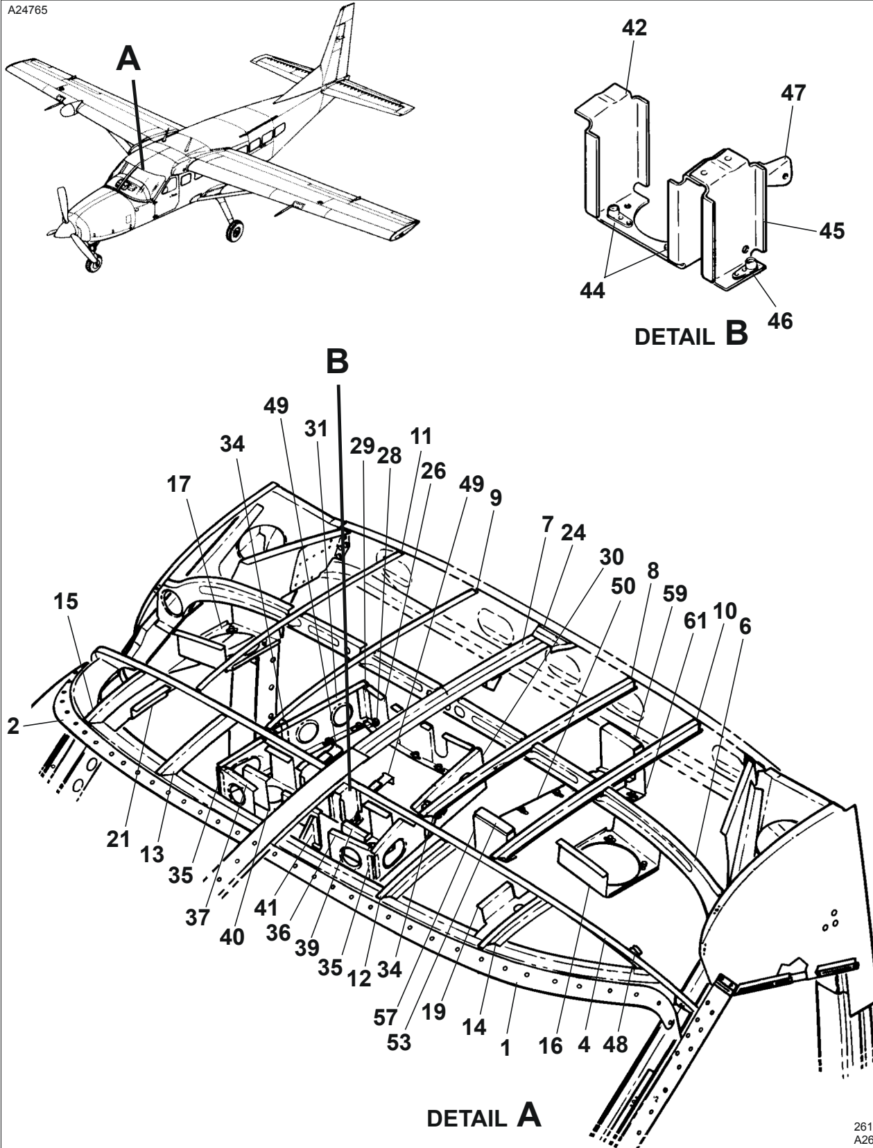
FORWARD CABIN TOP COMPONENTS Figure 03. (Sheet 1)
