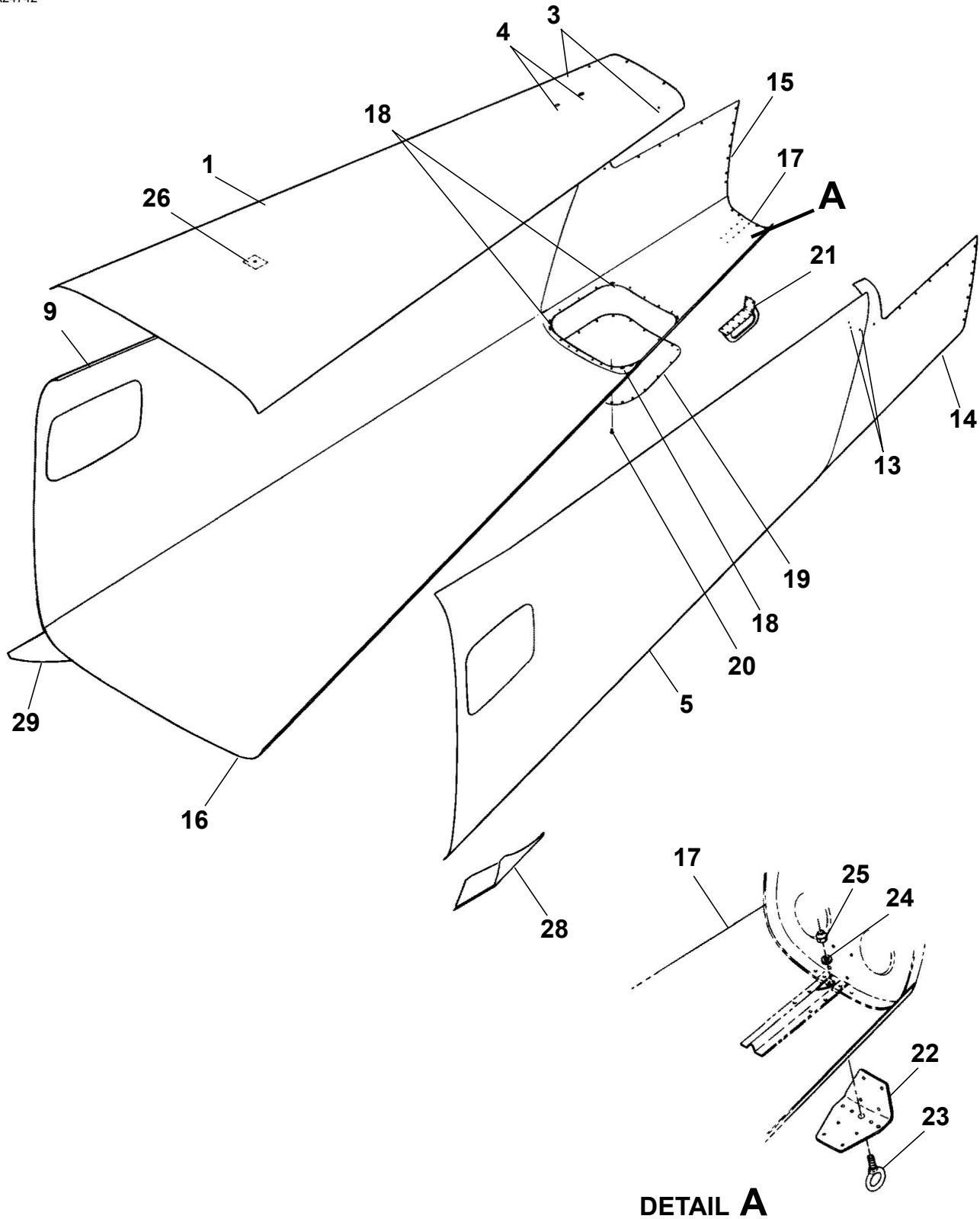
TAILCONE SKINS AND COMPONENTS Figure 01. (Sheet 1)
