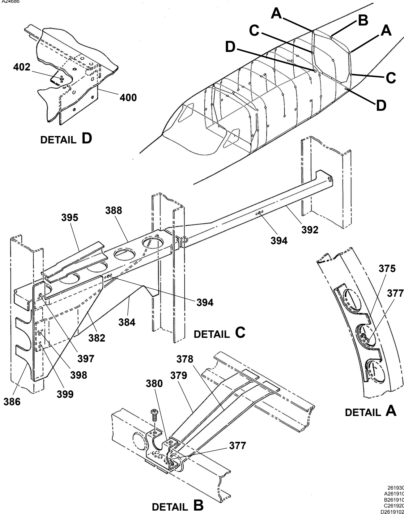
CARGO TIE DOWN STRUCTURE COMPONENTS Figure 02. (Sheet 6)
