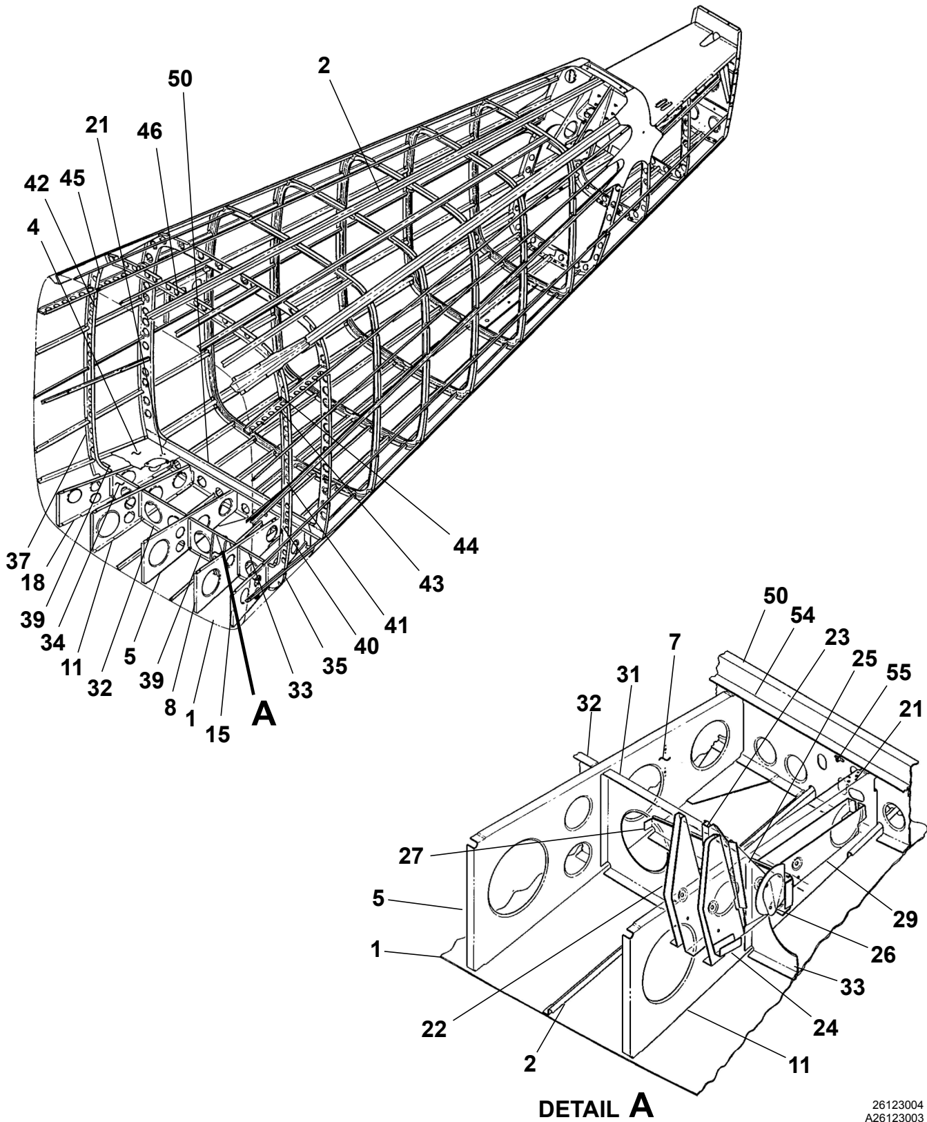
DETAIL A TAILCONE STRUCTURE - NOT APPLICABLE TO PASSENGER VERSION Figure 02. (Sheet 1)
