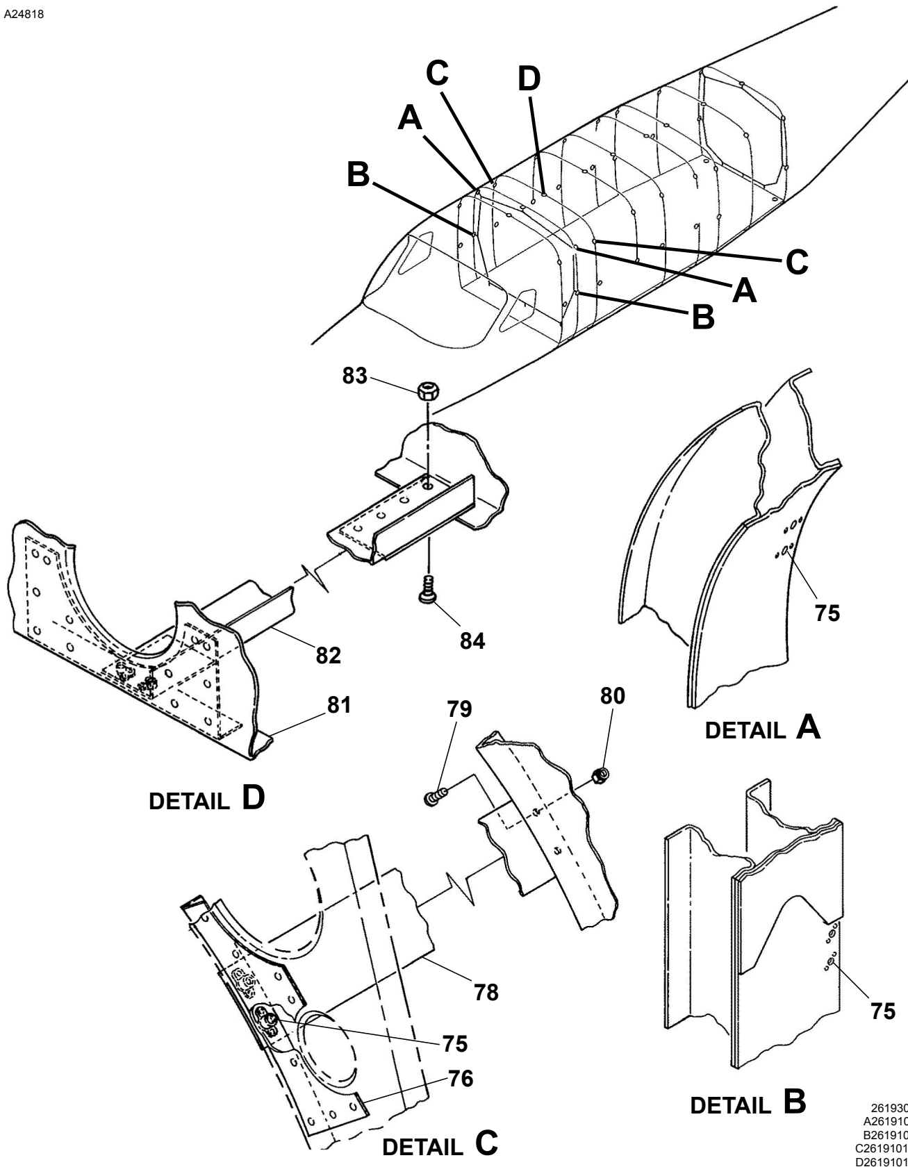
CARGO TIE DOWN STRUCTURE COMPONENTS Figure 02. (Sheet 2)
