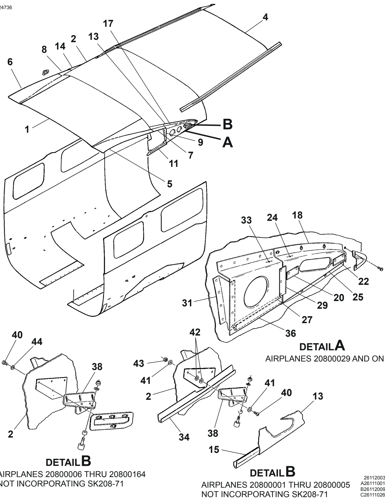
CENTER FUSELAGE SKINS AND COMPONENTS Figure 01. (Sheet 1)
