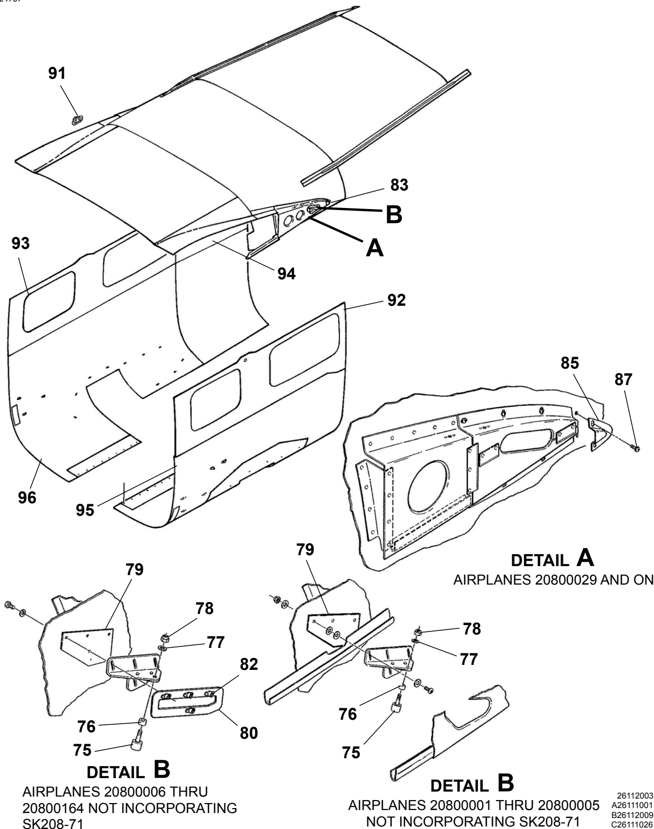
CENTER FUSELAGE SKINS AND COMPONENTS Figure 01. (Sheet 2)
