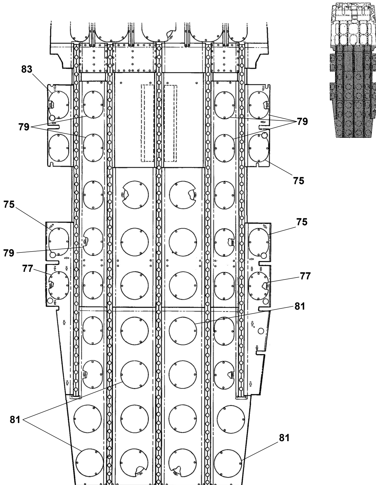
FLOORBOARD ACCESS PANELS Figure 01. (Sheet 2)
