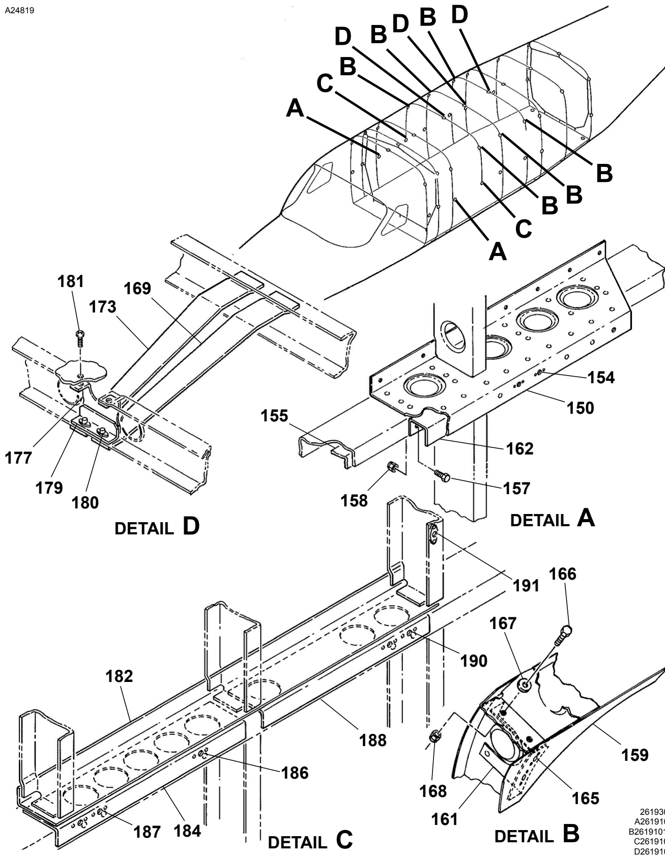
CARGO TIE DOWN STRUCTURE COMPONENTS Figure 02. (Sheet 3)
