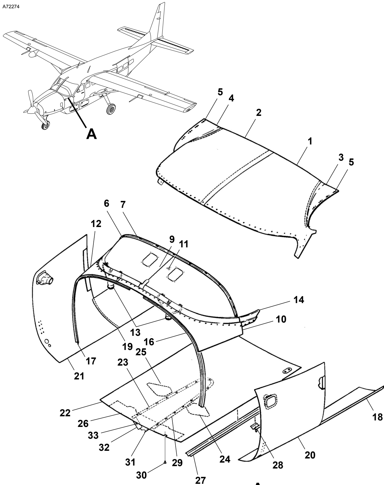
FORWARD FUSELAGE SKINS AND COMPONENTS Figure 03. (Sheet 1)
