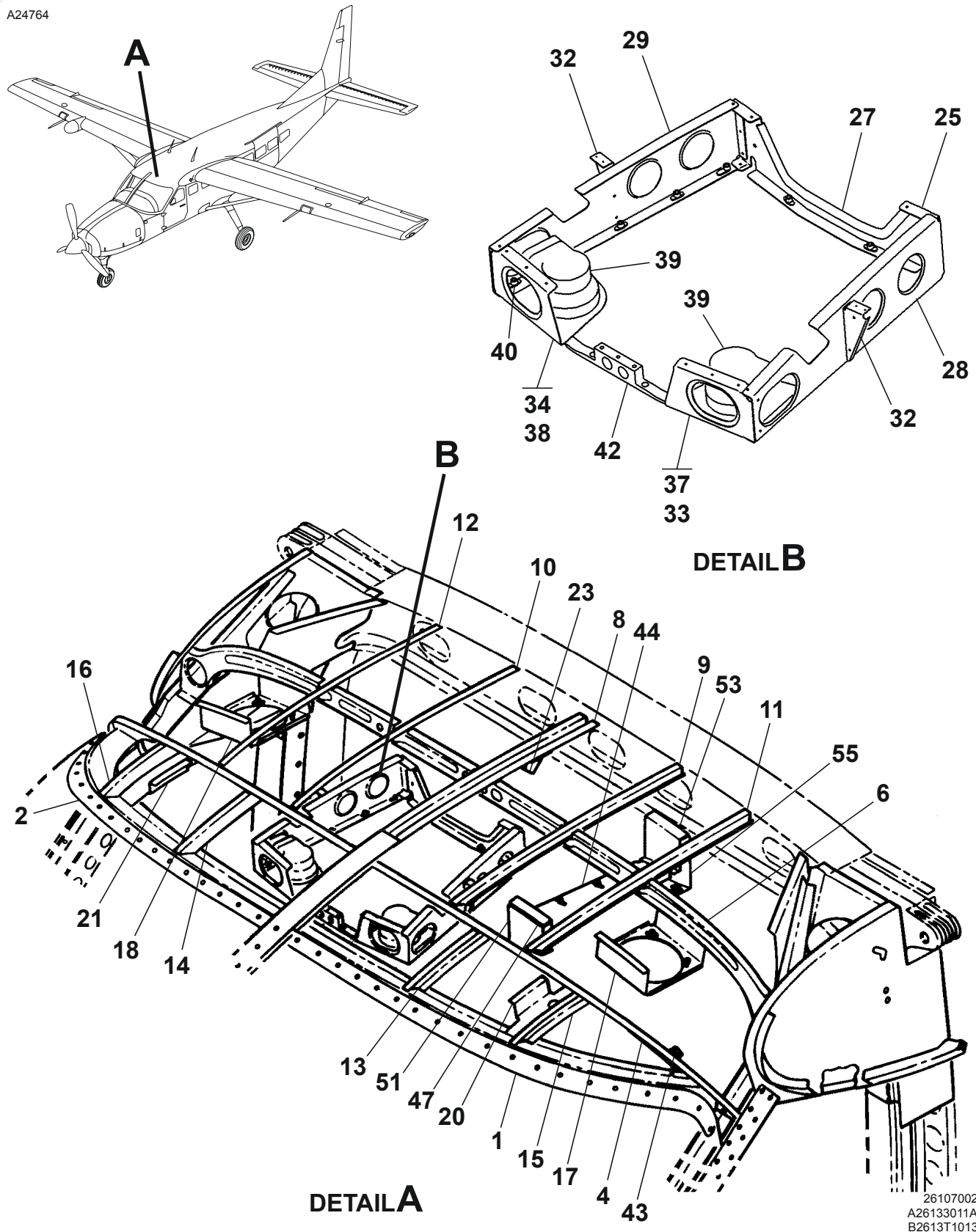
FORWARD CABIN TOP COMPONENTS Figure 02. (Sheet 1)
