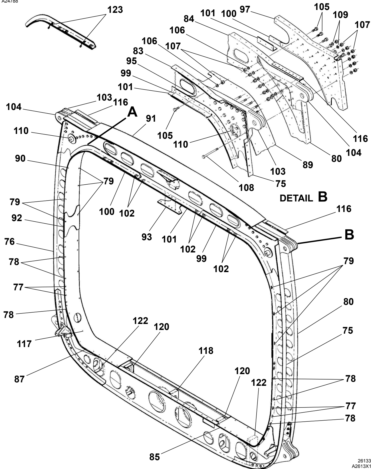
FORWARD CARRY-THRU STRUCTURE Figure 03. (Sheet 2)
