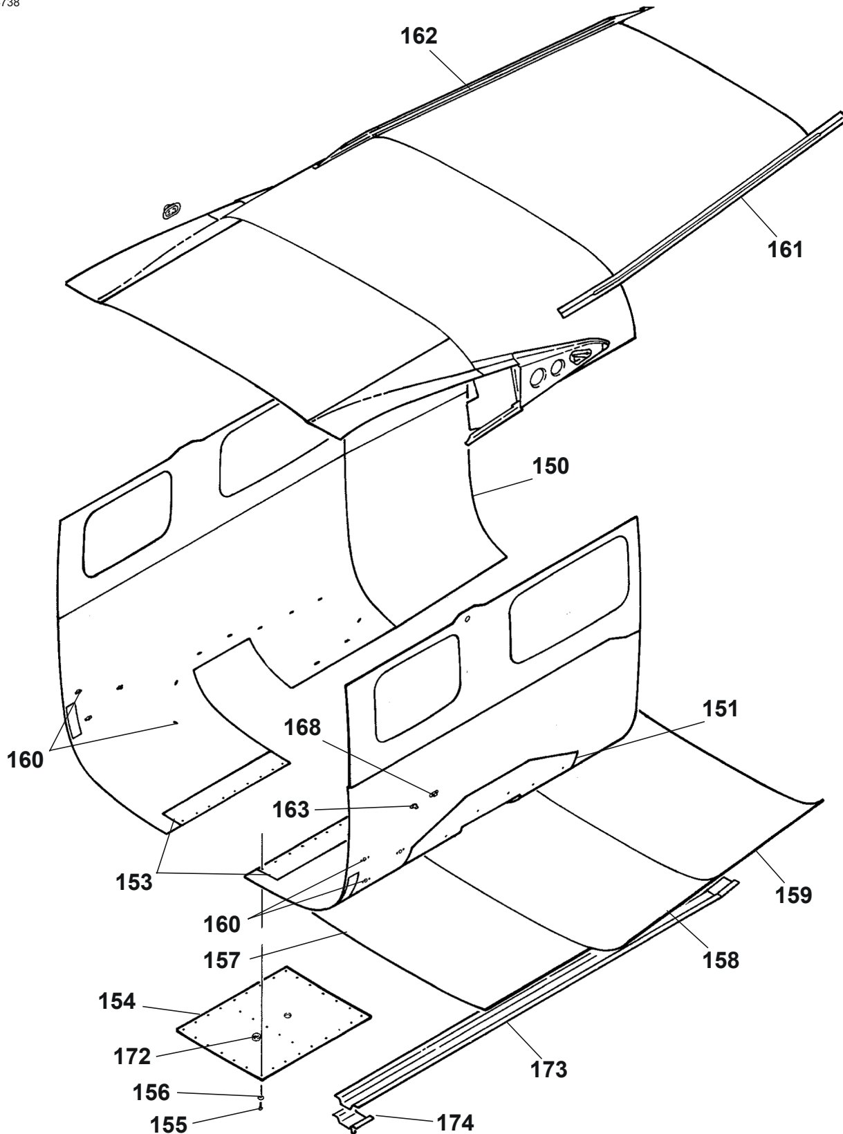
CENTER FUSELAGE SKINS AND COMPONENTS Figure 01. (Sheet 3)
