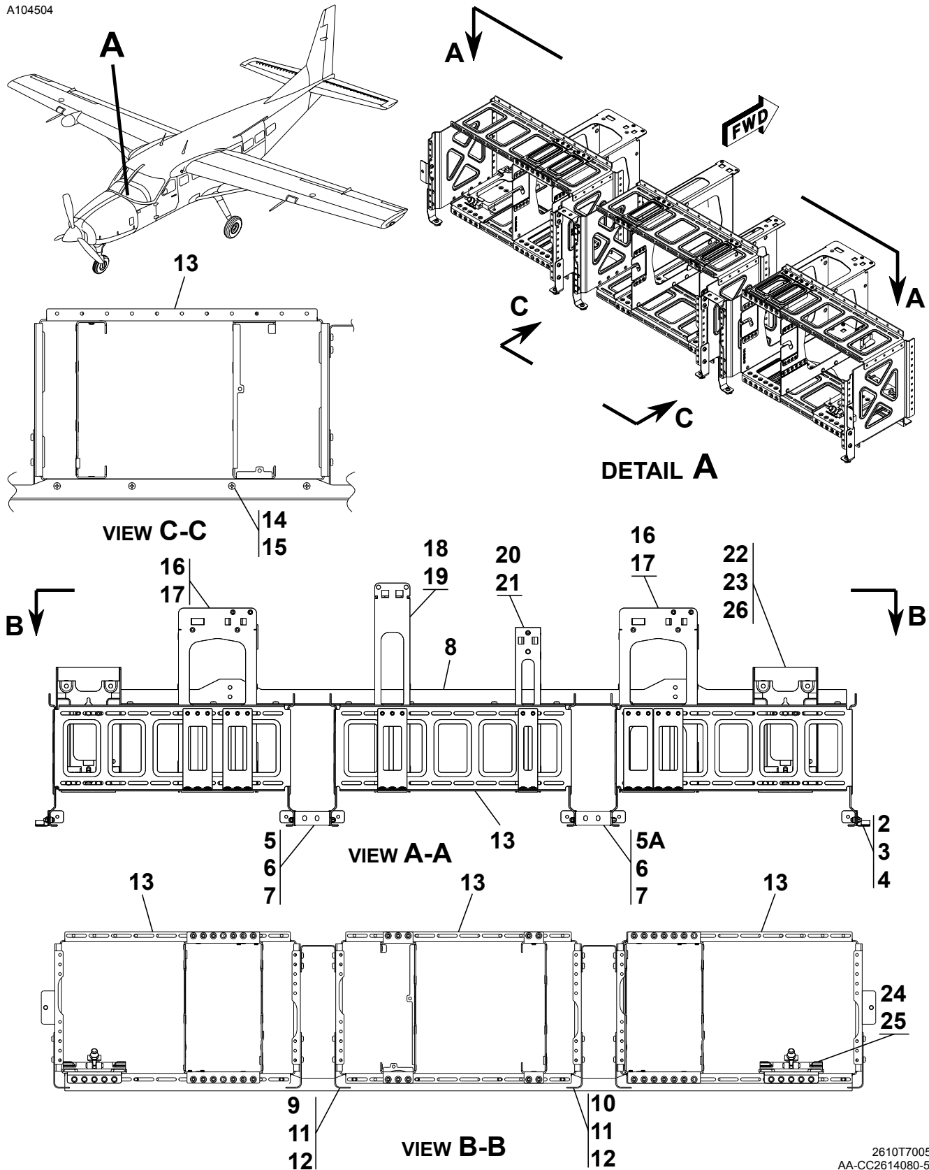
G1000 NXI RACK ASSEMBLY Figure 02. (Sheet 1)
